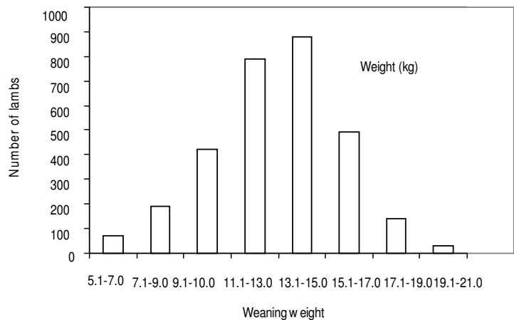
Fig. 6.1. Histogram of the distribution of weaning weight of Afar sheep.
